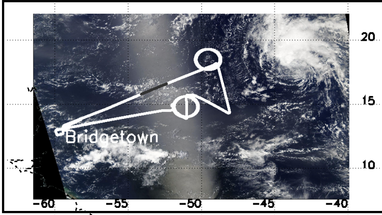
Figure 2. Flight track of HALO (redwhite) from RF 06 (19–19 August 2016) plotted on a METEOSAT-MODIS Terra satellite composite image from 19:30 UTC. The section for which the remote sensing measurements are analyzed (19:24 UTC to 19:39 UTC) crosses a region with aggregated trade wind cumulus and is plotted in greengray.
