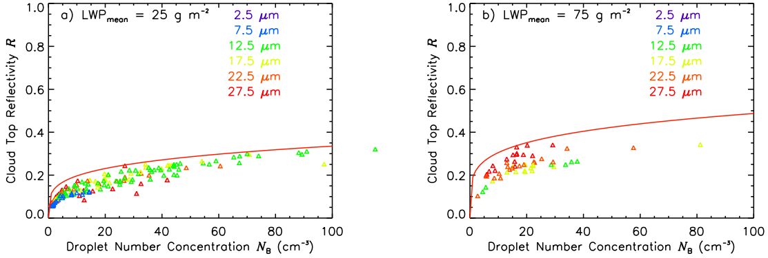
Figure 9. Cloud top reflectivity \mathcal{R}_{532} as a function of cloud droplet number concentration N_B for homogeneous, non-precipitating clouds of different liquid water path LWP_B (panel a: 0-50 \text{ g m}^{-2} , panel b: 50-100 \text{ g m}^{-2} ). The droplet effective radius r_{\text{eff}} of each measurement is indicated by the color code. The red line represents simulated reflectivity \mathcal{R}_{532} from radiative transfer calculations for clouds with same LWP .
