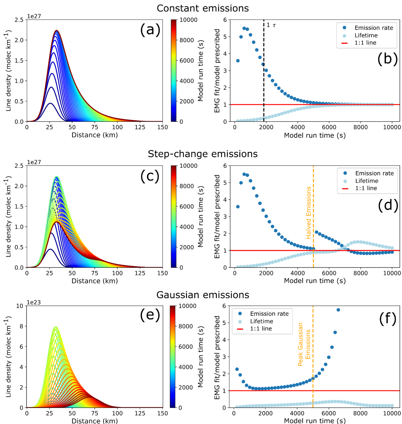
Figure 5: (a) Line densities of a hypothetical compound from a 1-D model with prescribed chemical lifetime of 30.8 minutes and constant emissions colored by model run time. (b) EMG fit / model prescribed emission rate (blue) and lifetime (light blue) at every model output step through the course of the entire model runtime. The model time equal to the model lifetime is indicated with a vertical, black dashed line. (c) Line densities for a 1-D model where the emission rate is halved halfway through the model runtime, colored by model run time. (d) Similar to (b), but for the model in (c). The vertical, gold dashed line indicates where the
