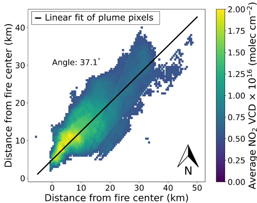
Figure A1: Time-averaged NO 2 VCD plume, where plume pixels were more than 3 times greater than the NO 2 upwind background. The black line is a linear fit of the plume pixels, where the standard deviation at each location was the difference between the maximum NO 2 VCD and the location's NO 2 VCD. The angle of the line is displayed.
