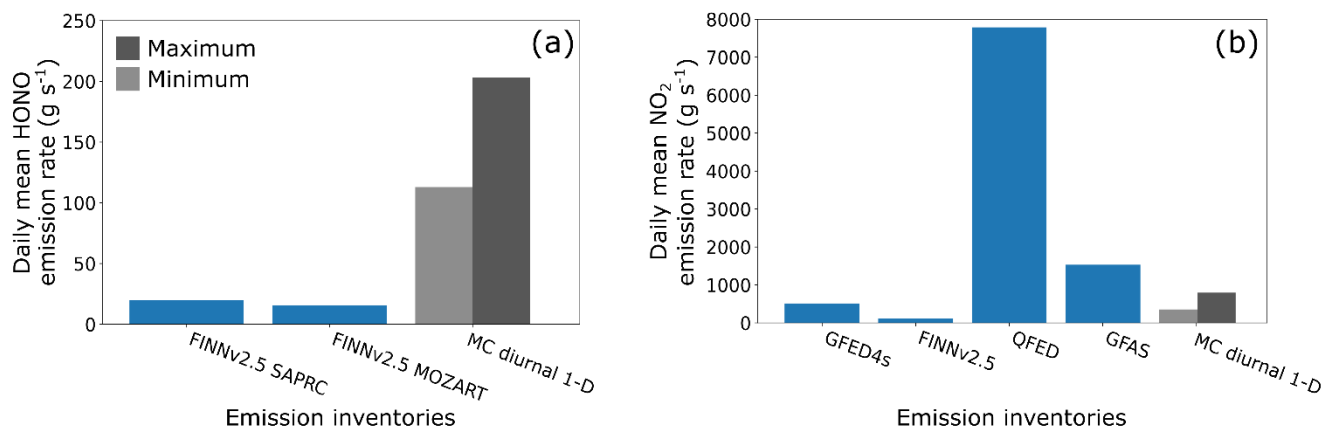
Figure 7: Daily mean emissions of (a) HONO and (b) \text{NO}_2 from the Monte Carlo diurnal 1-D model method (MC diurnal 1-D) using the R^2 = 0.9 contour to define the minimum and maximum emissions, and the following biomass burning emission inventories: FINNv2.5 SAPRC, FINNv2.5 MOZART, GFED4s, FINNv2.5, QFEDv2.5, and GFASv1.2.
